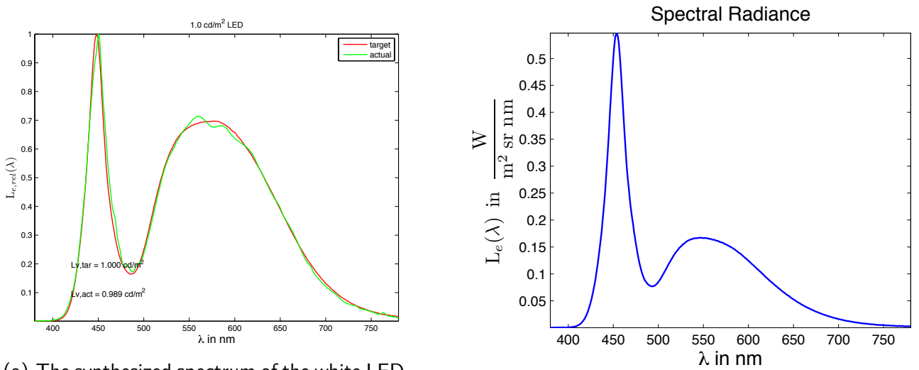
(a) The synthesized spectrum of the white LED with a S/P ratio of 1.71 and a CCT of 4322 K.
